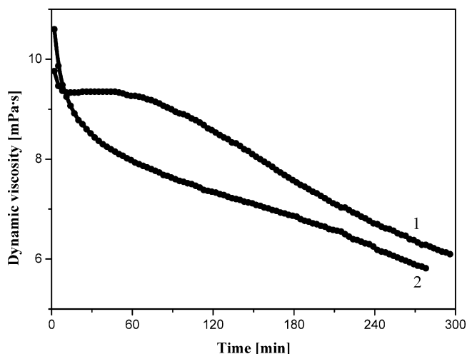
Figure 3. Kinetics of degradation of high-molecular-weight HA (2.5 mg/mL) induced by the combined action of 0.1 \mu M Cu^{2+} and 100 \mu M ascorbic acid (curve 1) and of 0.1 \mu M Cu^{2+} , 100 \mu M ascorbic acid, and 5.0 mM HOCl (curve 2).
